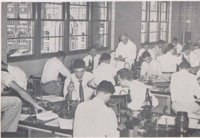
Splitting the atom.
